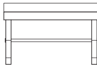
Luggage Bench OXB-3620 36"W x 20"D x 20"H
