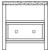
24" Nightstand OXN-2418 24"W x 18"D x 25"H
