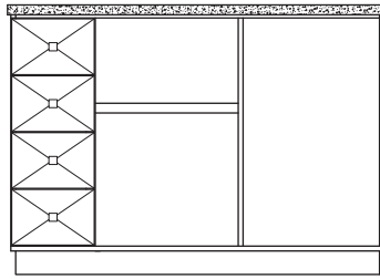
Service Unit (shown with granite option) OXU-5824 58½"W x 24"D x 41½"H
