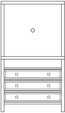
Dresser with TV Panel Mount for Flat Screen OXTV-3622 36"W x 22"D x 62"H
