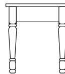
End Table PVT-2224 22"W x 24"D x 25"H
