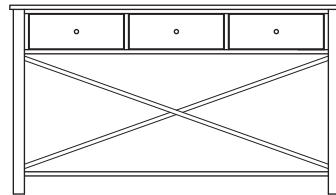
Console Table CC-01 60"W x 18"D x 34"H
