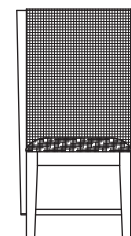
Armless Dining Chair PPDR-02 22 1/2"W x 22"D x 41 1/2"H
